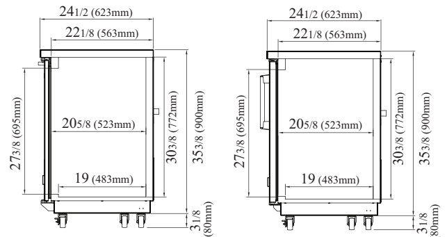
TBB-24-72SBD-N6 & TBB-24-72SGD-N SIDE VIEW
