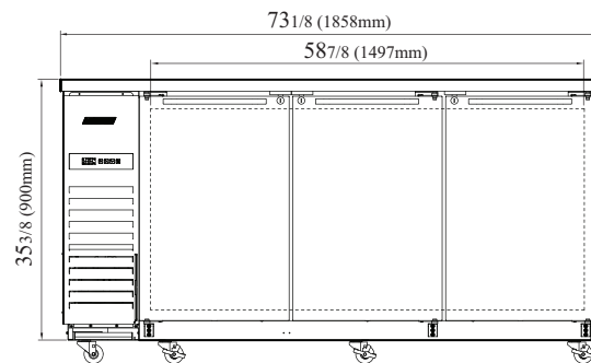
TBB-24-72SBD-N6 FRONT VIEW
