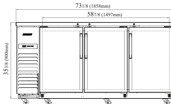
TBB-24-72SGD-N FRONT VIEW
