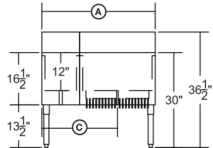
Front View - Cold plate models
