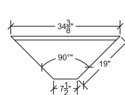
KR19-R90
