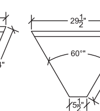
KR24-R60
