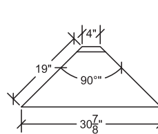
KR19-F90
