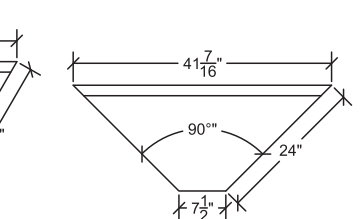
KR24-R90
