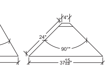
KR24-F90
