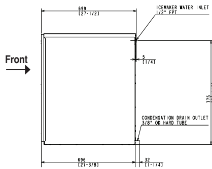
WATER-COOLED
