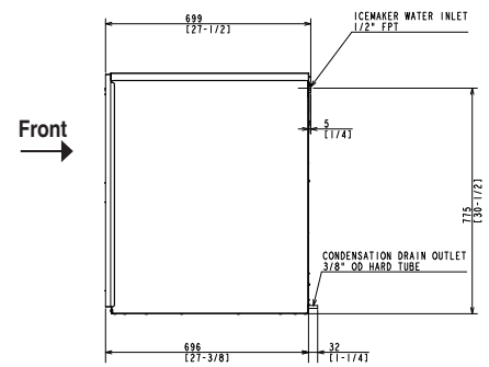
REMOTE AIR-COOLED
