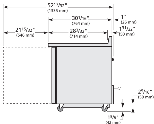
RIGHT VIEW
